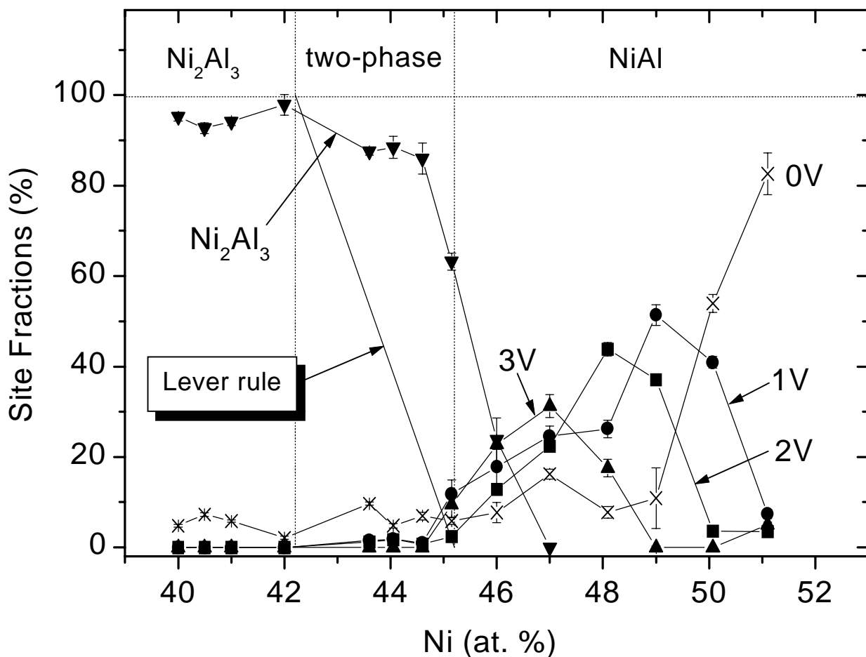
Fig. 3. Site fractions of In impurities in Ni-Al alloys. For the NiAl phase, fractions are shown for probes having 0, 1, 2 or 3 near-neighbor Ni-vacancies. For the Ni_2Al_3 phase is shown the sum of fractions for all its sites.
