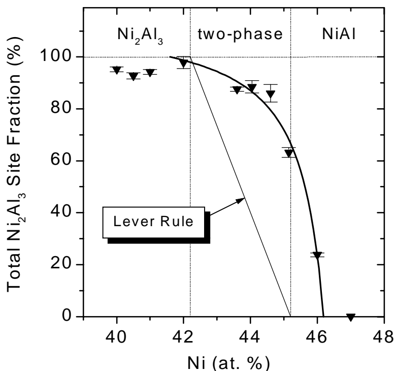
Fig. 4. Site fraction of probes in the Ni 2 Al 3 phase as a function of composition. The curve is from a fit of the data to eq. 2 under the assumption that the probes are segregating to that phase.
