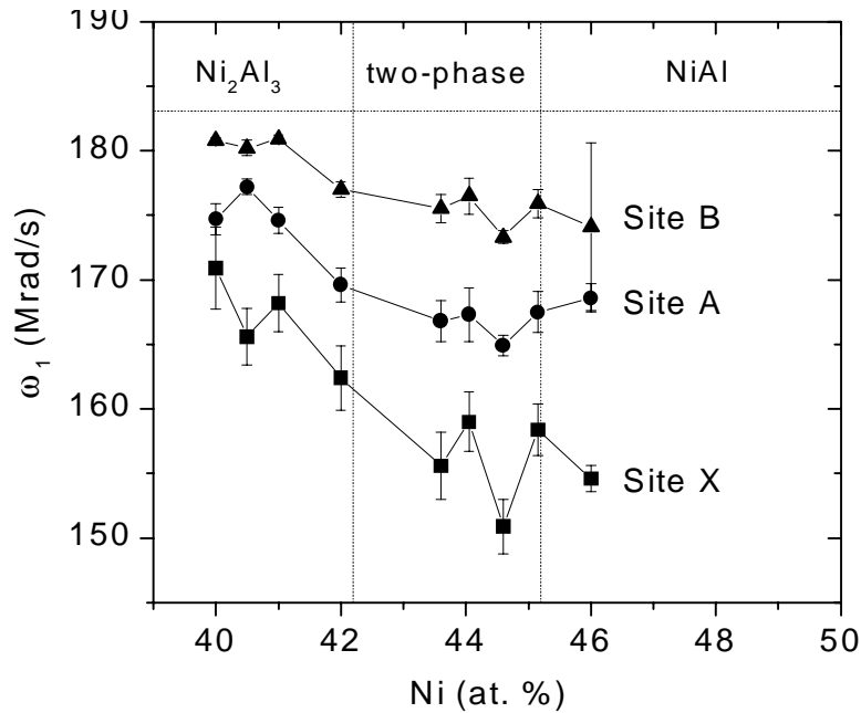
Fig. 5. Composition dependence of quadrupole interaction frequencies of the three signals detected in the Ni_2Al_3 phase
